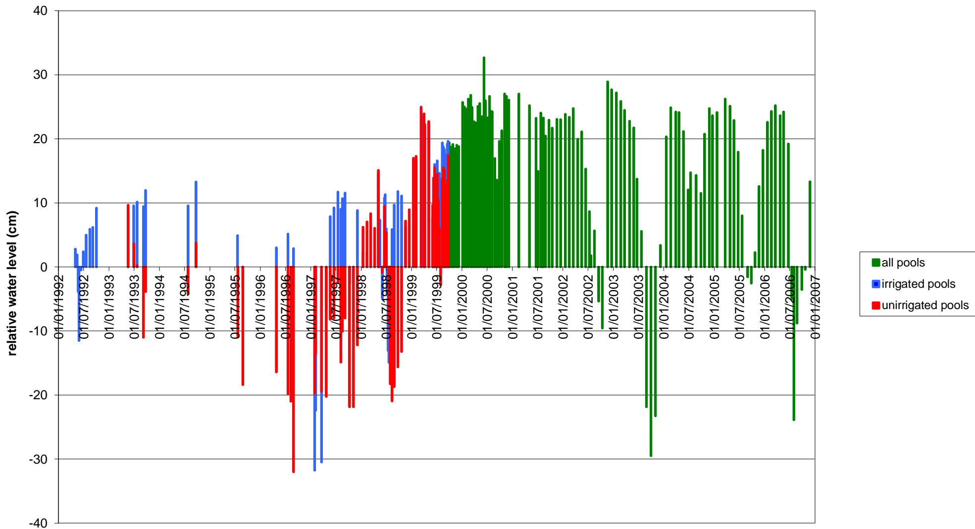
Fig. 7 Water levels in Little Fen ponds 1992-2006. Horizontal line represents the April 1992 datum. Blue and red lines represent mean levels in irrigated and unirrigated ponds respectively: summer irrigation stopped in 1999 (see text).
