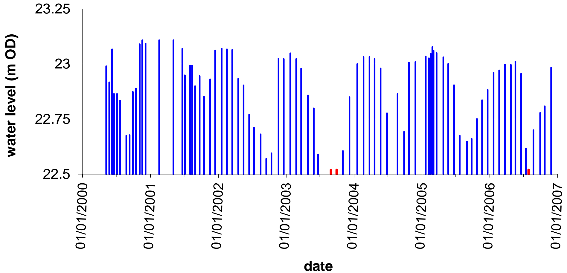
Fig. 10 Water levels in ponds excavated on Great Fen in 1998. Broken line denotes level below which most ponds are dry. Red indicated dates on which all ponds were completely dry.
