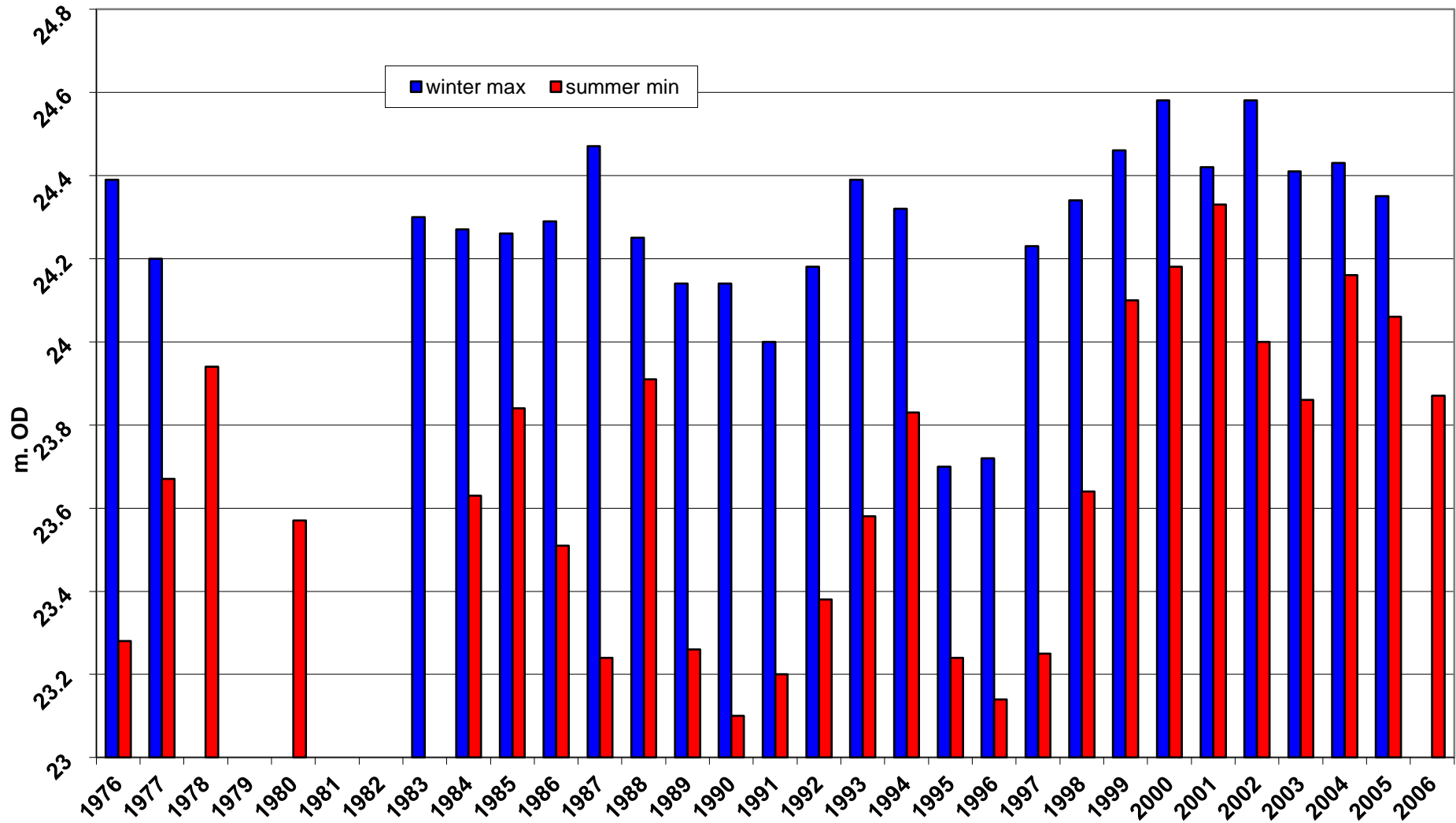
Fig. 6 Mean winter maximum and summer minimum water levels in piezometers on Redgrave and Lopham Fen NNR
