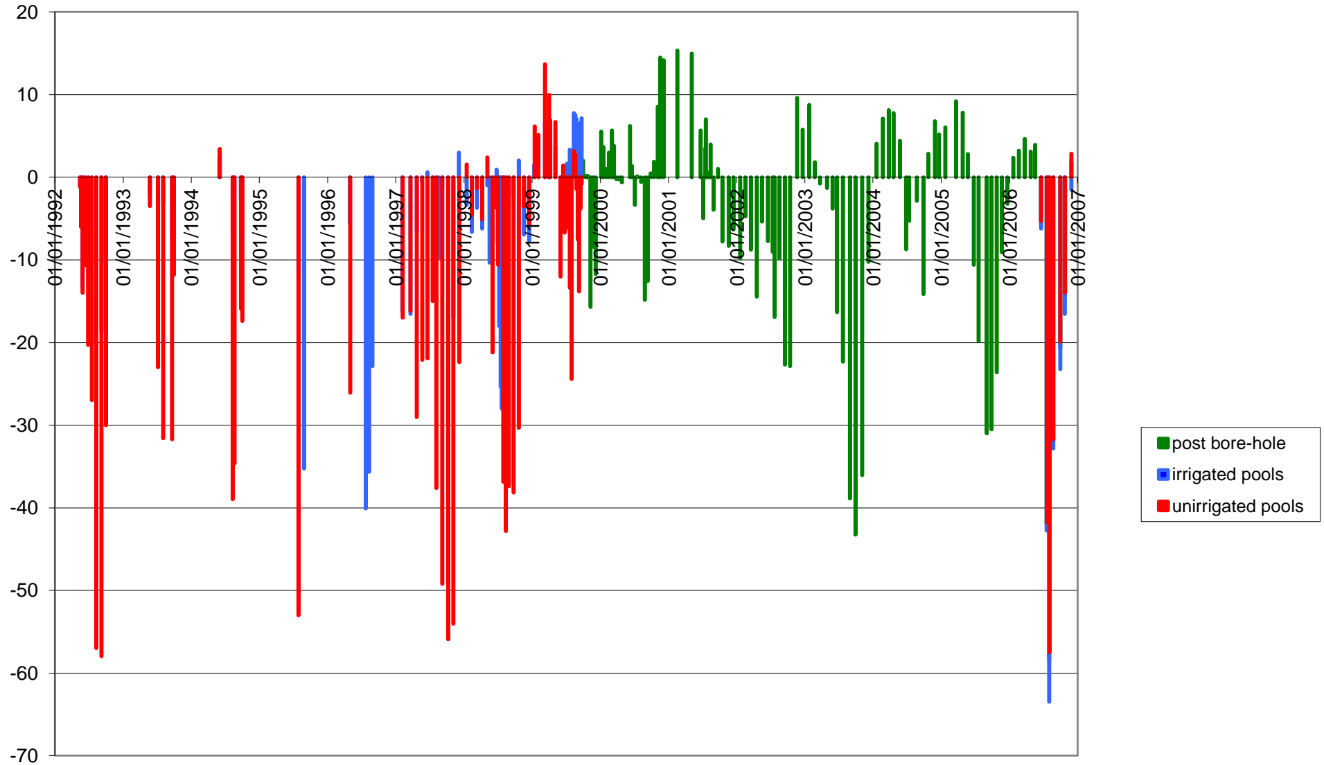
Fig. 8 Water levels in Middle Fen ponds 1992-2006. Horizontal line represents the April 1992 datum. Blue and red lines represent mean levels in irrigated and unirrigated ponds respectively: summer irrigation stopped in 1999 but differences between the two sets of ponds are shown again for 2006 (see text).
